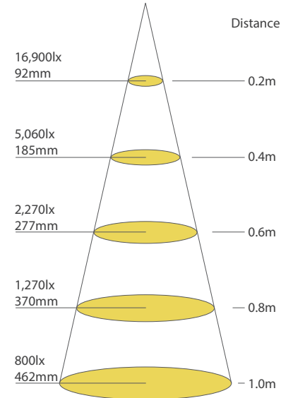
TANA Spot HCRI with 26° lens
