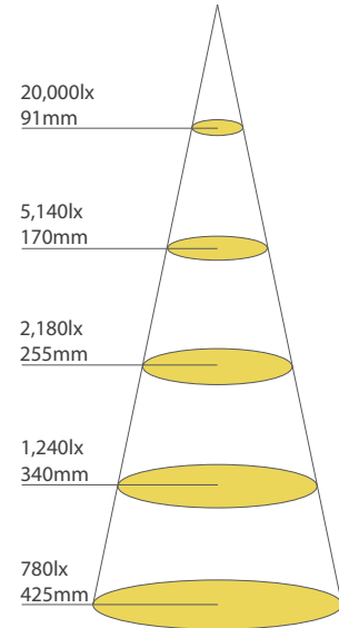
TANA Spot with 24° lens
