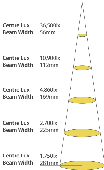
TANA Spot with 16° lens
