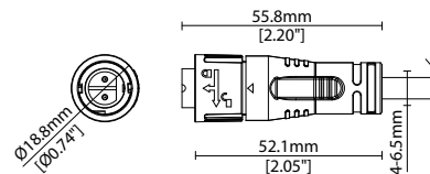
2 Pin Male Connector IP67 (Premoulded)
