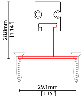
KKBK-05 Adjustable bracket (allow 2 per metre/40in) S/Steel finish
