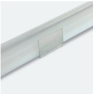
KKCP-05 (1no.) KKCP-55 (500no.) For use with KKLN-01 lens only Lens lock clip (allow 3 per metre/40in) Clear polycarbonate finish L25/W15.6/H24mm (L0.98/W0.61/H0.94")
